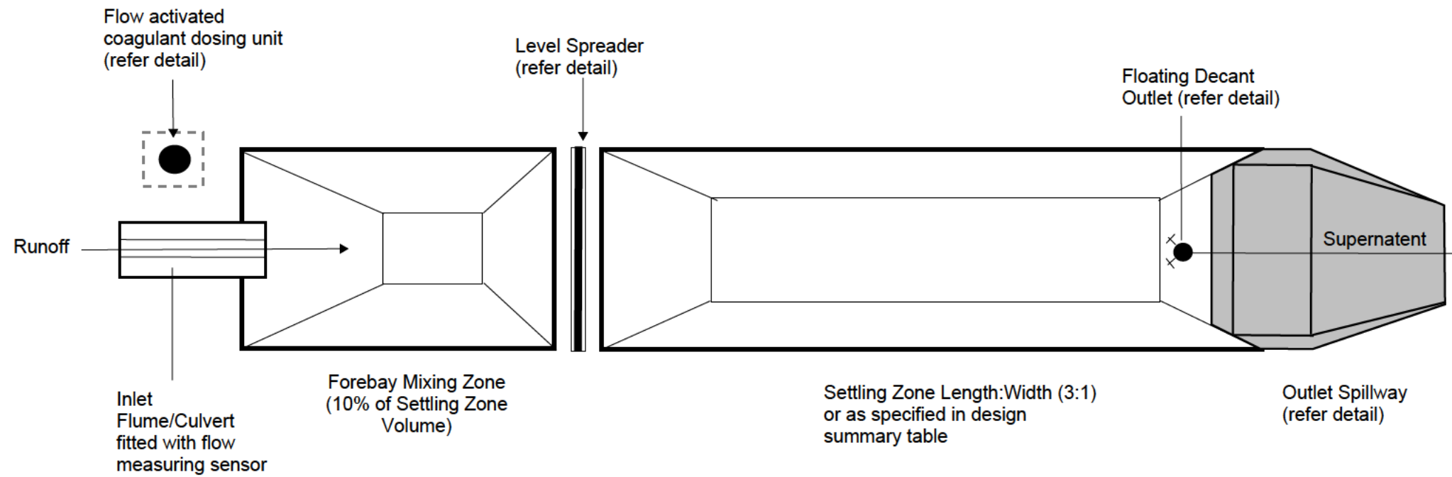
Type A Sediment Basin Plan View (Typical NTS)
