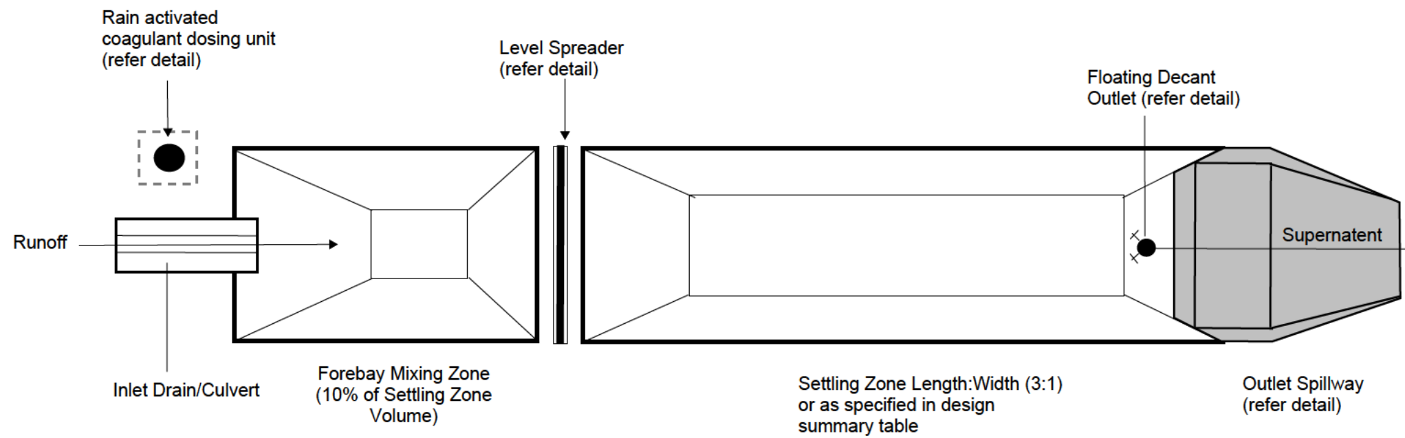
Type A Sediment Basin Plan View (Typical NTS)
