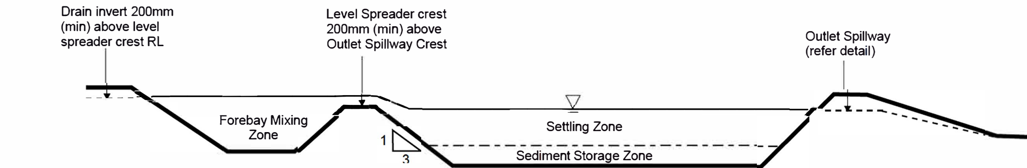
Type B Sediment Basin Long Section (Typical NTS)
