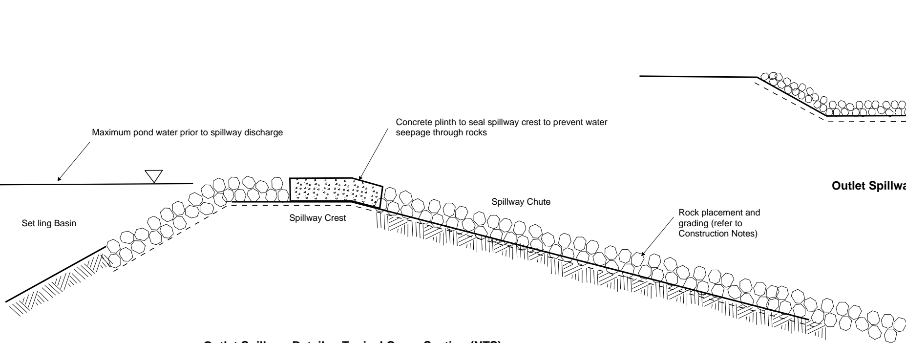
Outlet Spillway Details - Typical Cross Section (NTS)
