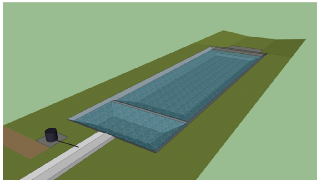
Basin Perspective (looking downstream)
